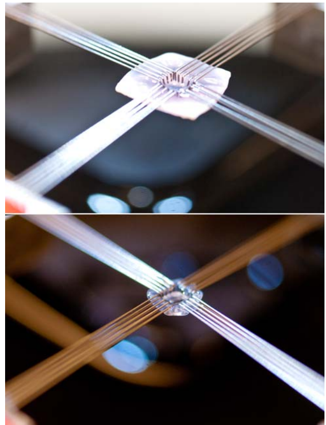
Figure 2 Fitting of the corneal specimens (top) and the flap (bottom) on the BioTester device.
